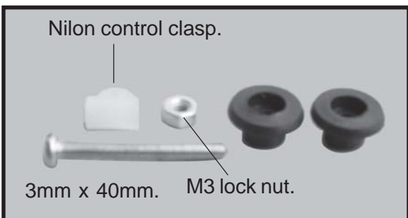
Control horn of Rudder.
